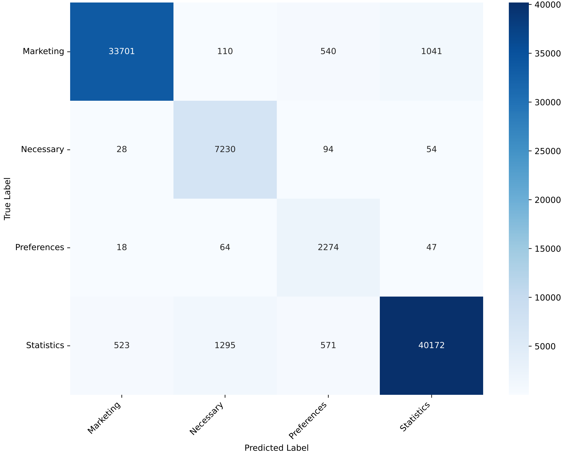
Confusion Matrix - Ridge Clasifier CV Test Accuracy: 95.00%
