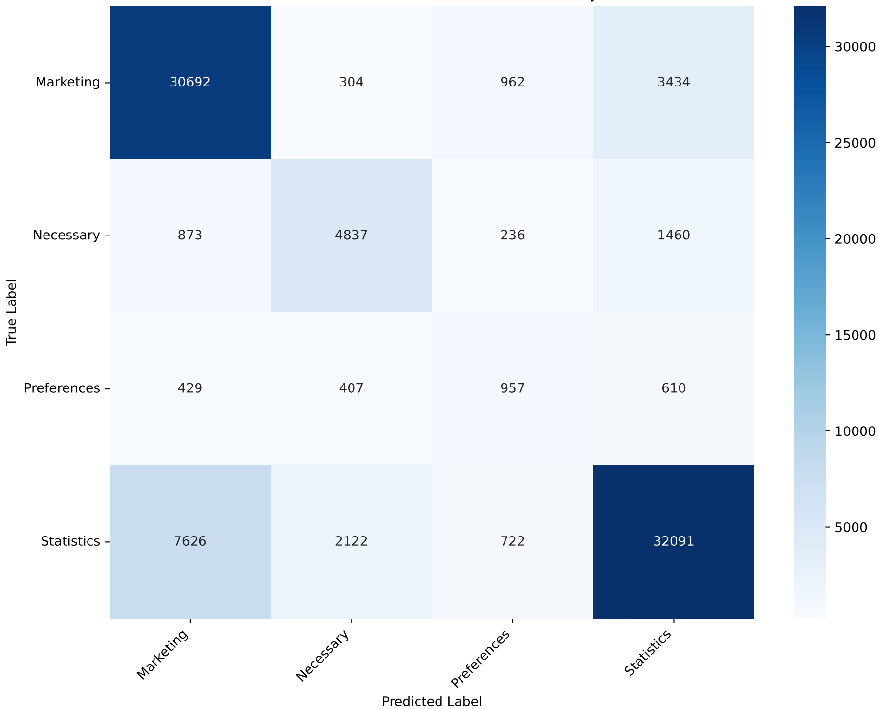
Confusion Matrix - Nearest Centroid Test Accuracy: 78.14%
