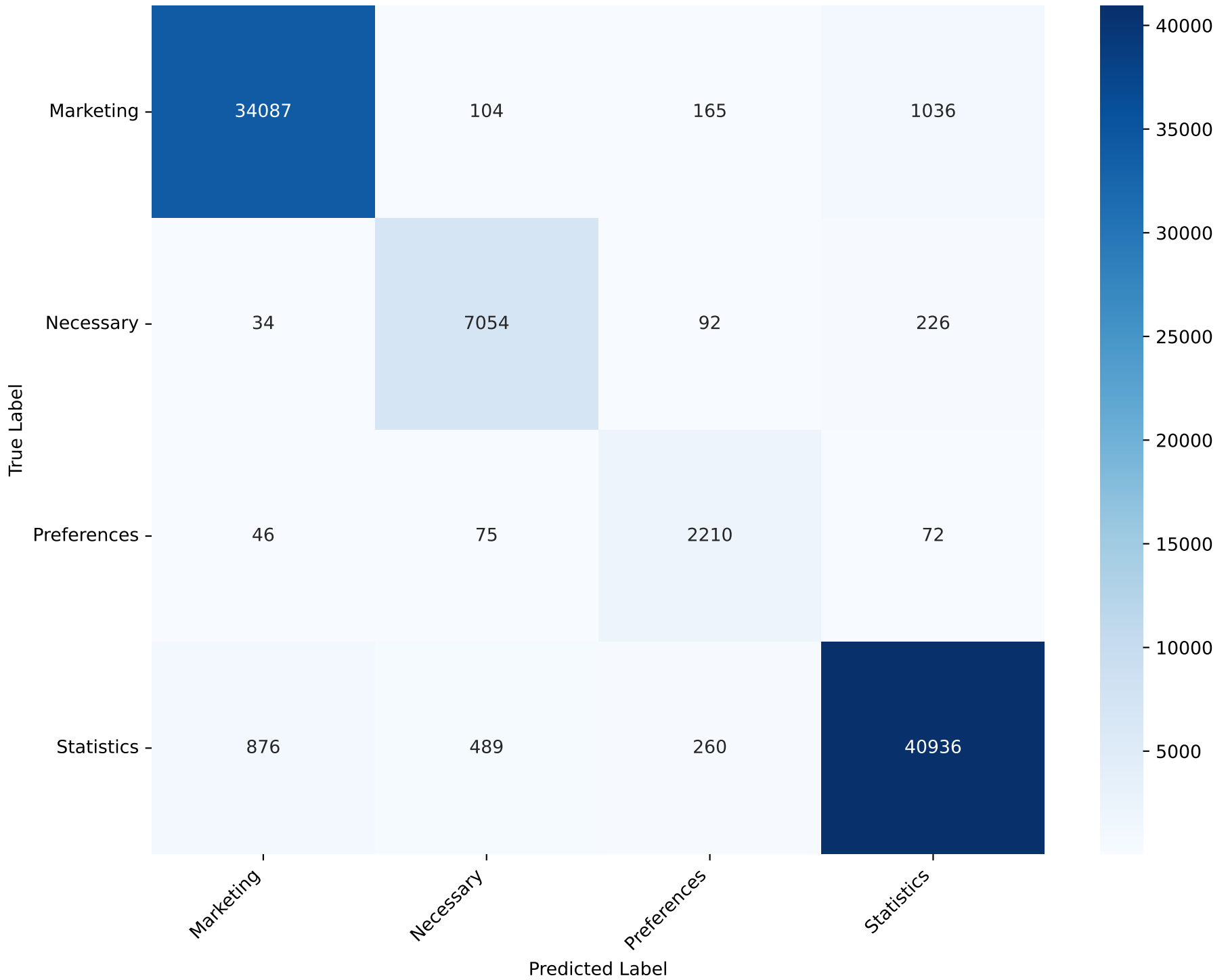
Confusion Matrix - Perceptron Test Accuracy: 96.04%
