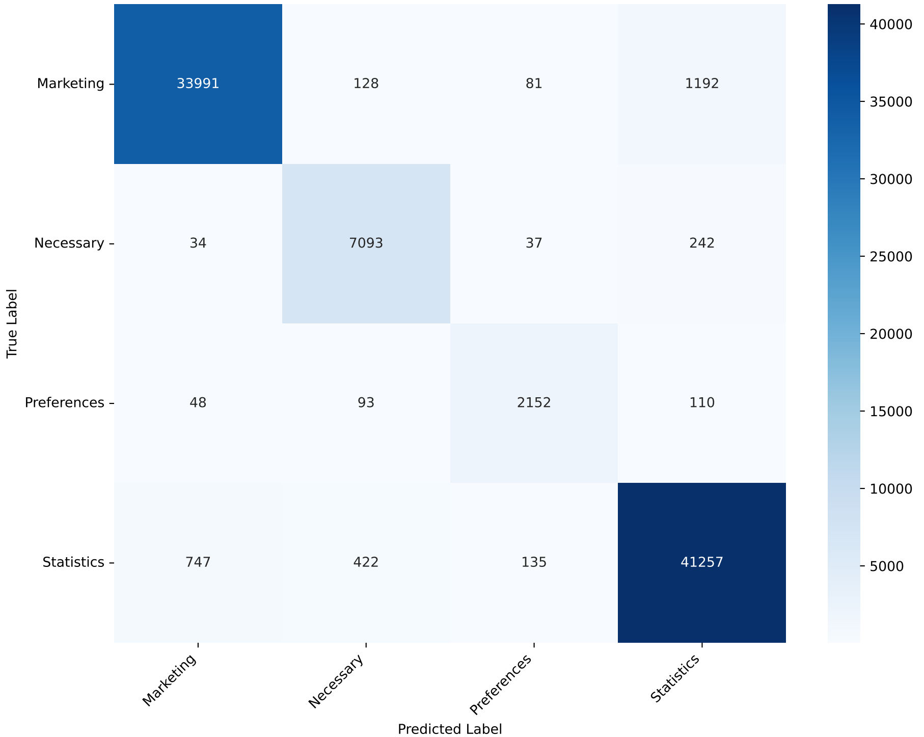
Confusion Matrix - Perceptron With Manual Weights Test Accuracy: 96.28%
