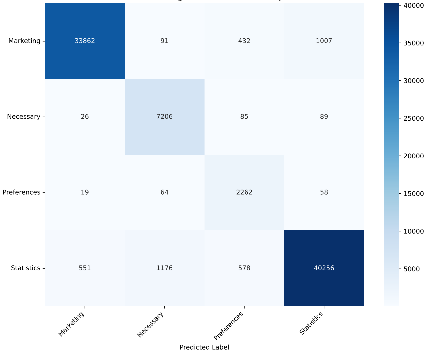
Confusion Matrix - Ridge CClassifier Test Accuracy: 95.24%
