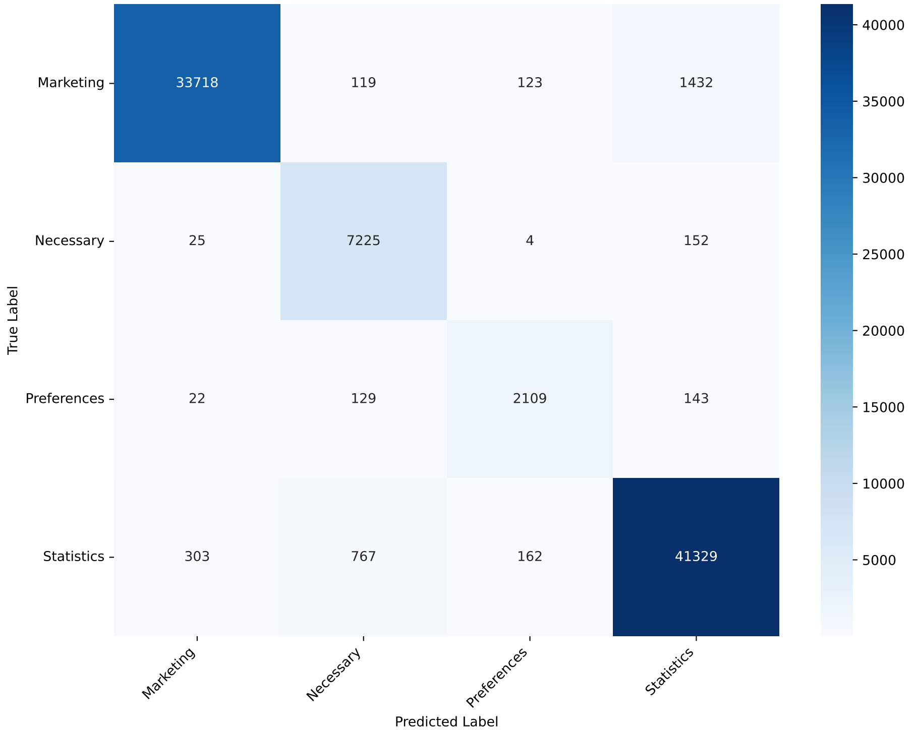
Confusion Matrix - Ridge CClassifier Manual Weights Test Accuracy: 96.15%
