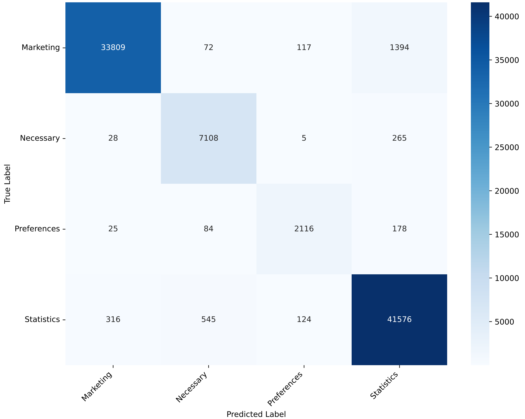
Confusion Matrix - Ridge CClassifier With Manual Weights Test Accuracy: 96.41%
