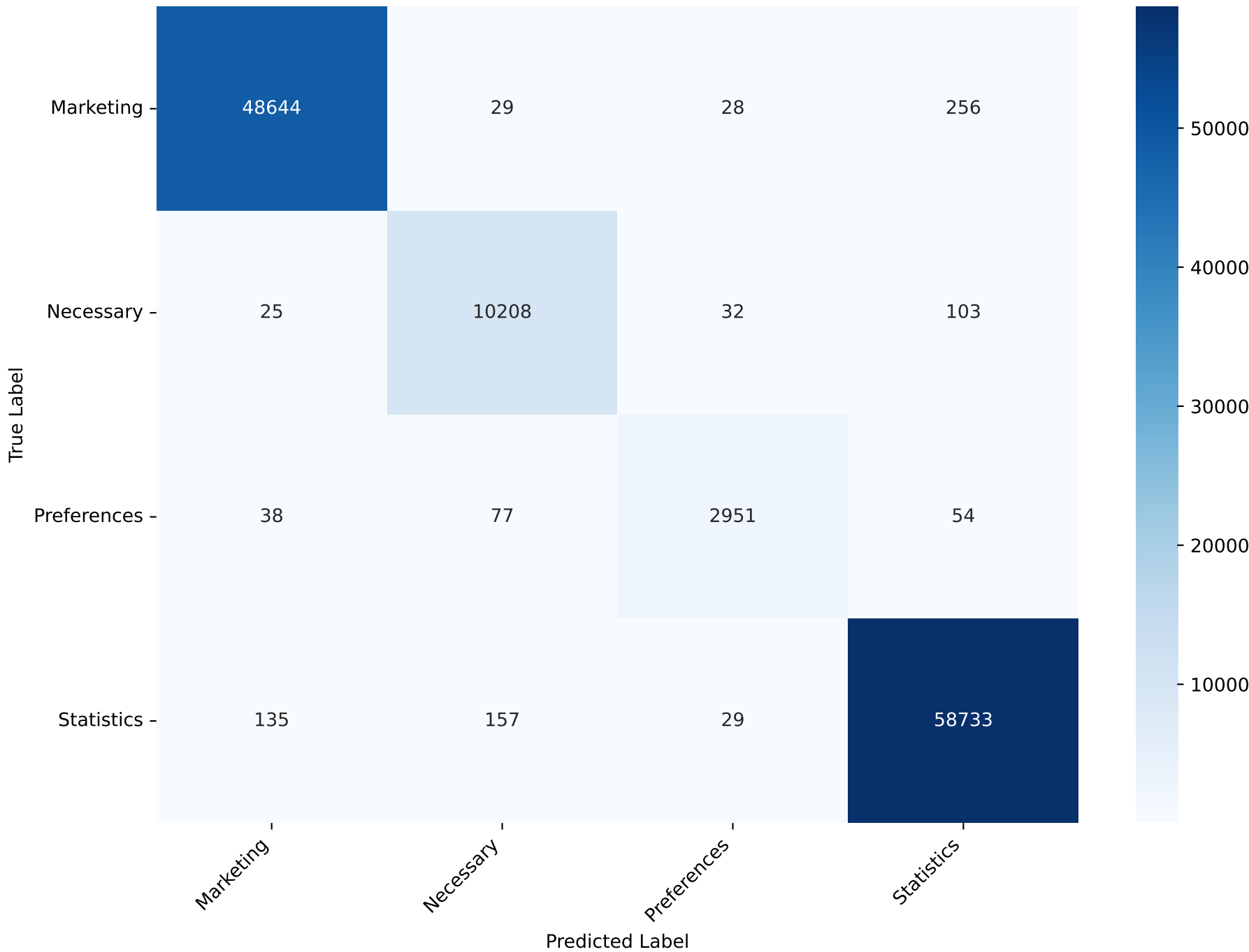
Confusion Matrix - MLP Test Accuracy: 99.21% Test F1 (macro): 98.16
