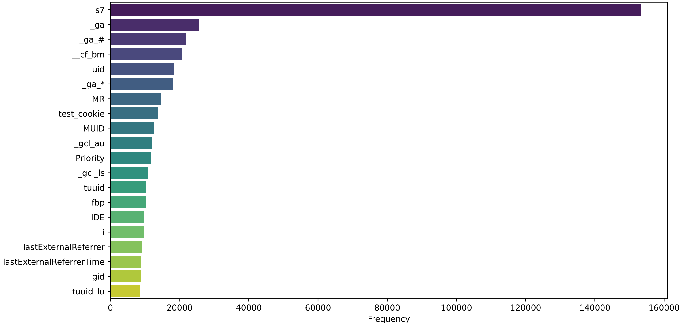
Top 20 Most Frequent Cookie Names
