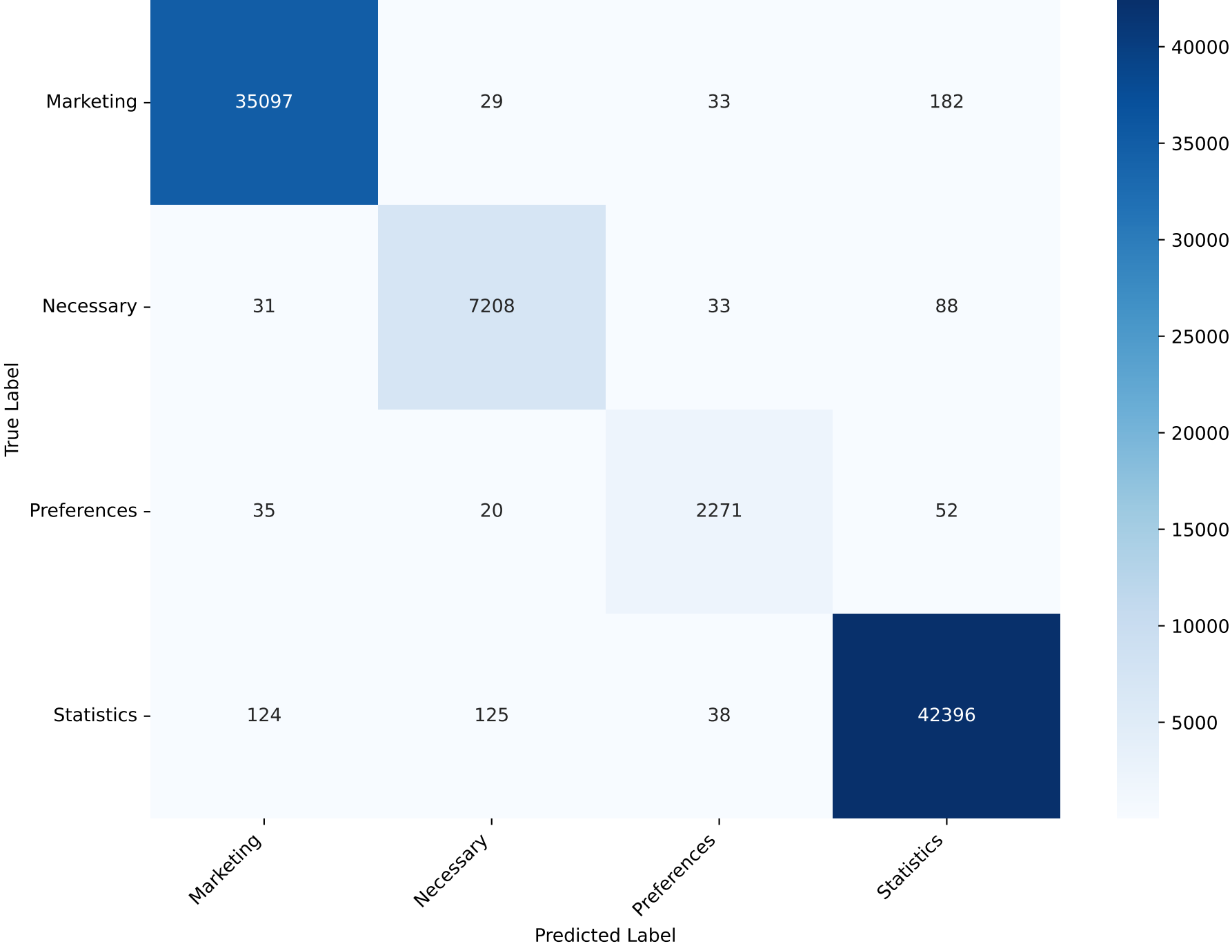
Confusion Matrix - MLP Test Accuracy: 99.10% Test F1 (macro): 98.01
