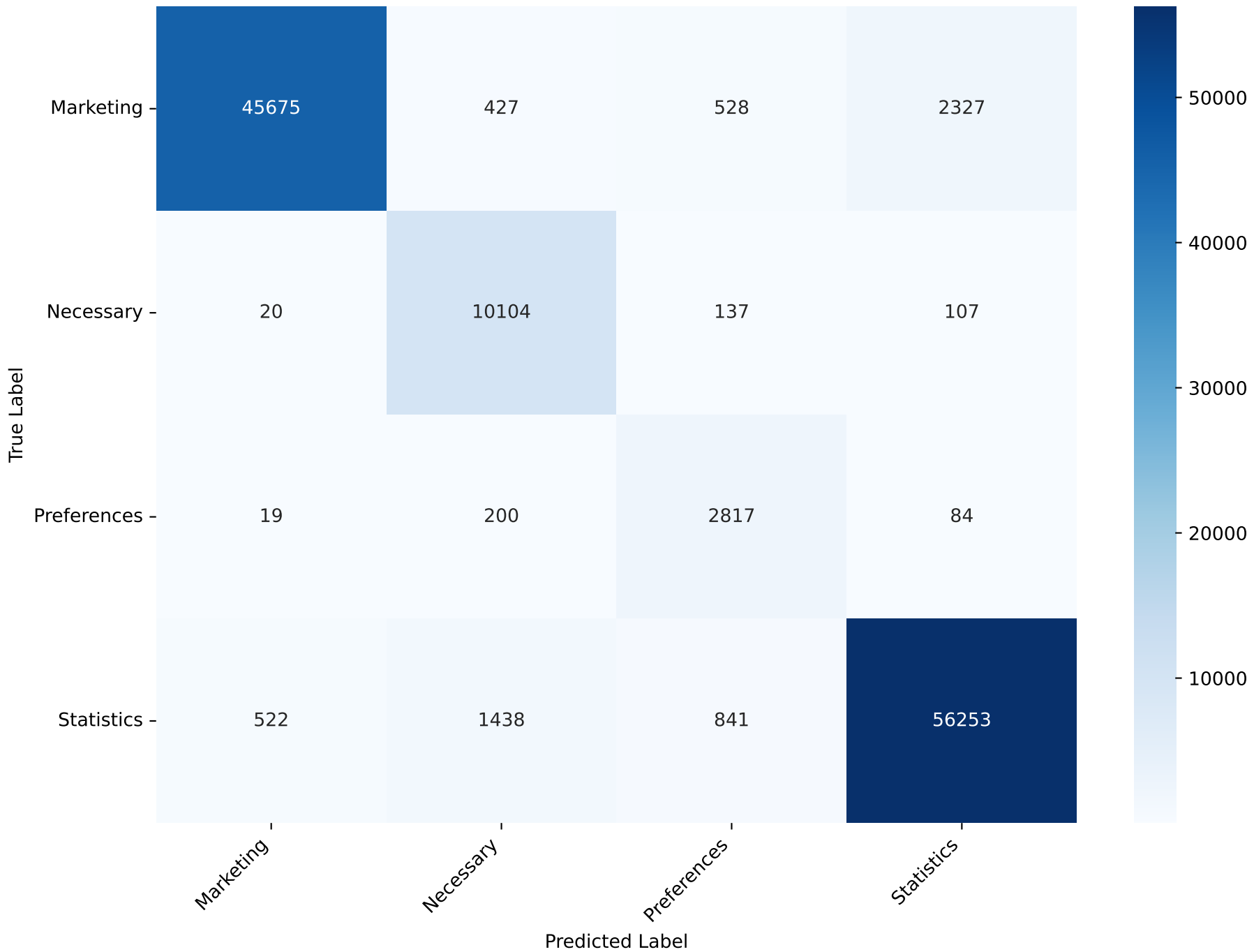
Confusion Matrix - LogisticRegression Test Accuracy: 94.53% Test F1 (macro): 89.20
