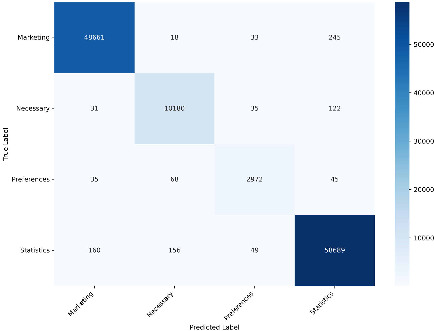
Confusion Matrix - MLP Test Accuracy: 99.18% Test F1 (macro): 98.12
