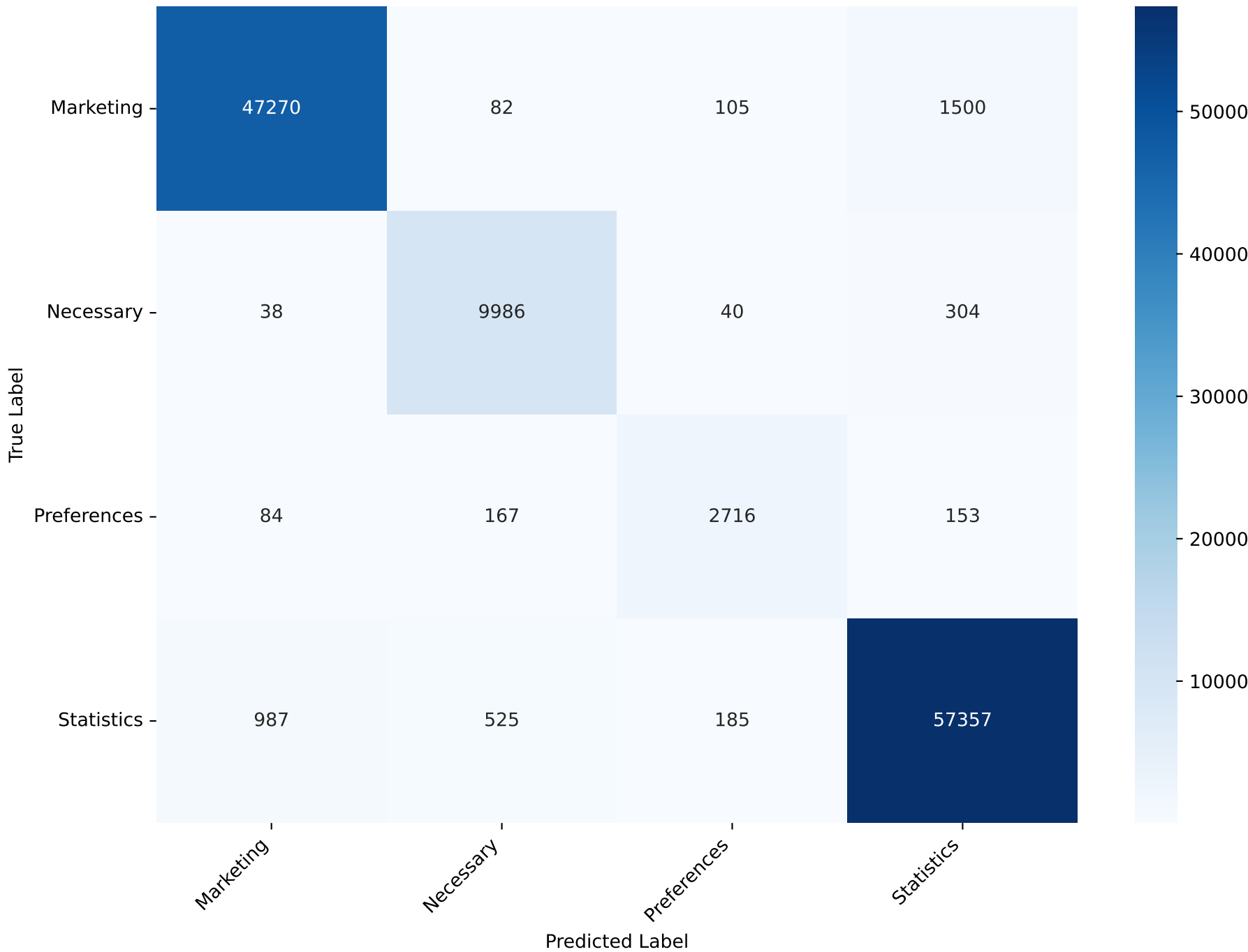
Confusion Matrix - PAC Test Accuracy: 96.57% Test F1 (macro): 94.17
