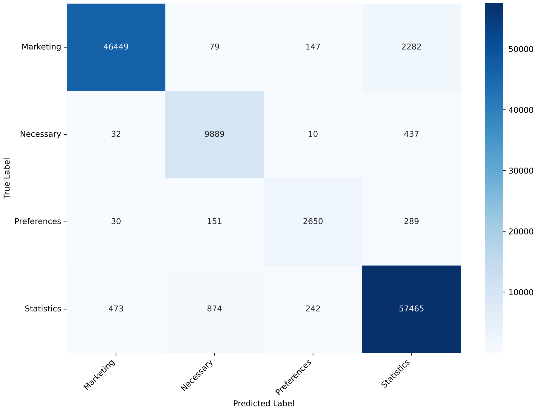
Confusion Matrix - RidgeClassifier_MW
