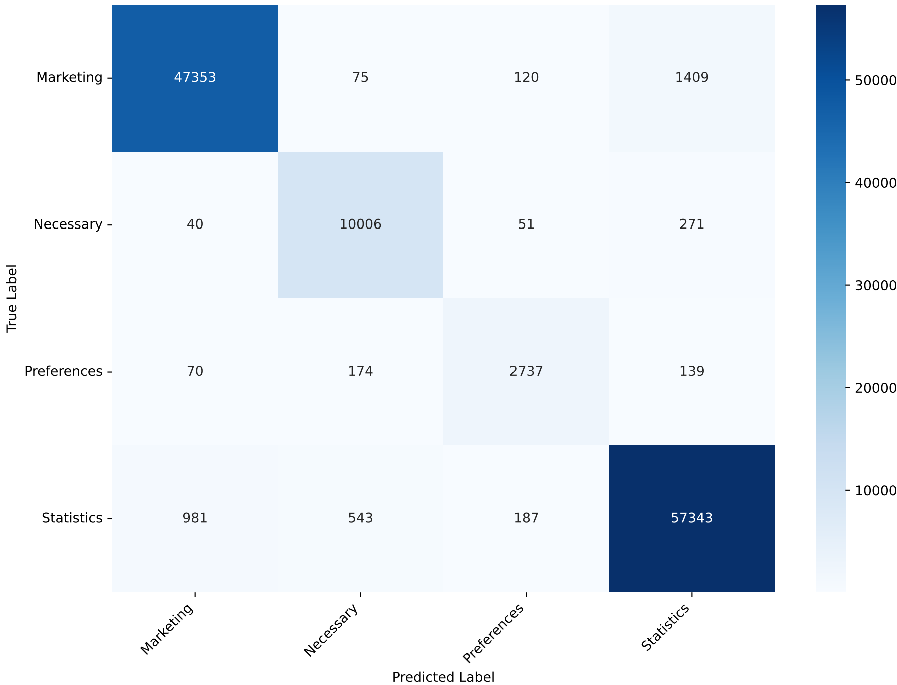
Confusion Matrix - SGD Test Accuracy: 96.66% Test F1 (macro): 94.22
