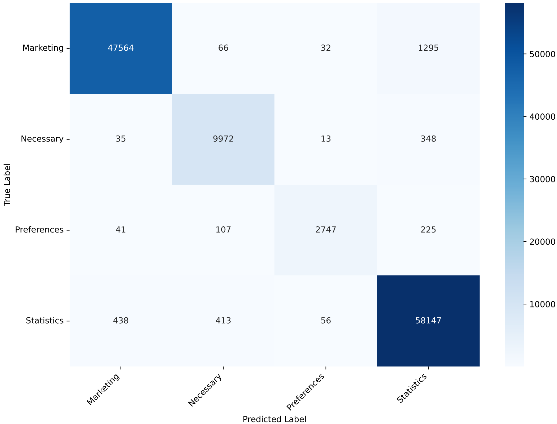
Confusion Matrix - XGBoost Test Accuracy: 97.47% Test F1 (macro): 95.77
