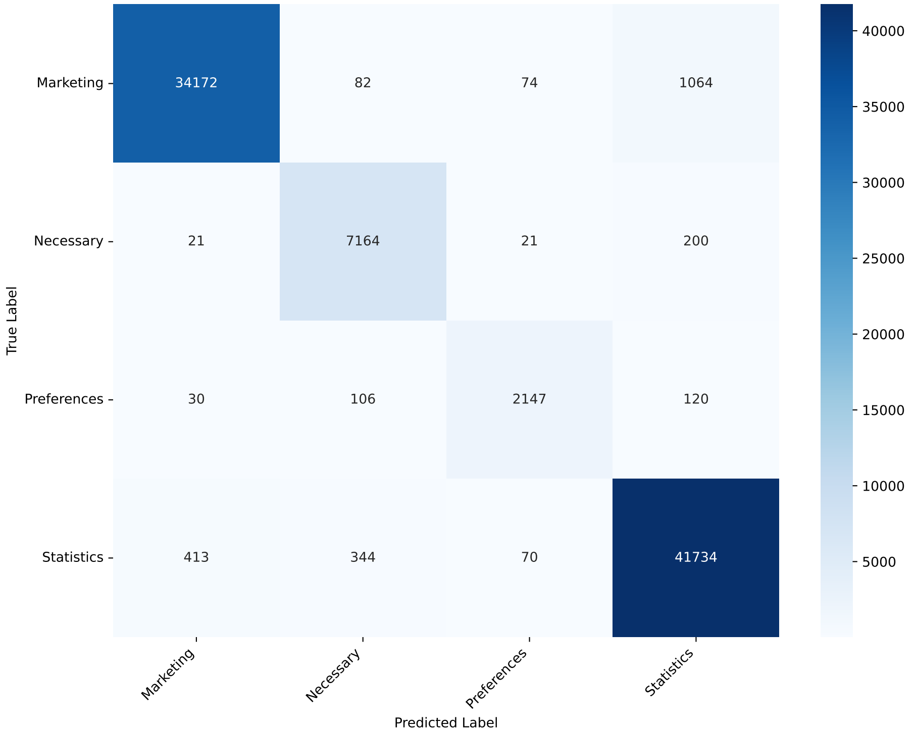
Confusion Matrix - LinearSVC Test Accuracy: 97.10%
