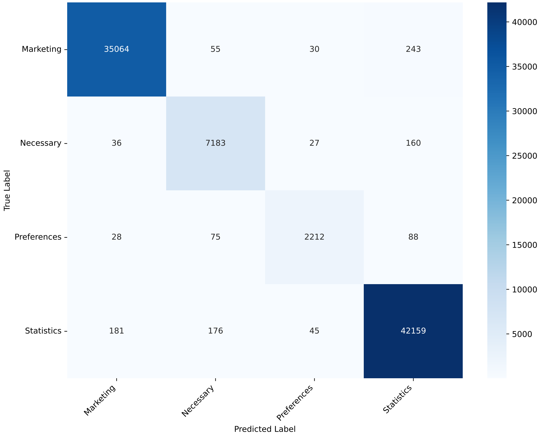
Confusion Matrix - MLP Classifier Test Accuracy: 98.70%
