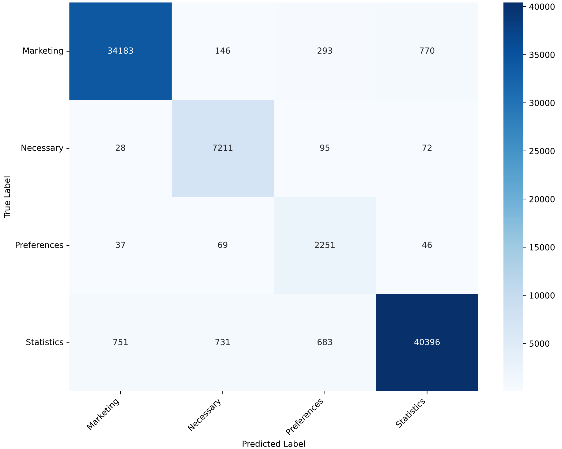
Confusion Matrix - Stacking Classifier Test Accuracy: 95.76%
