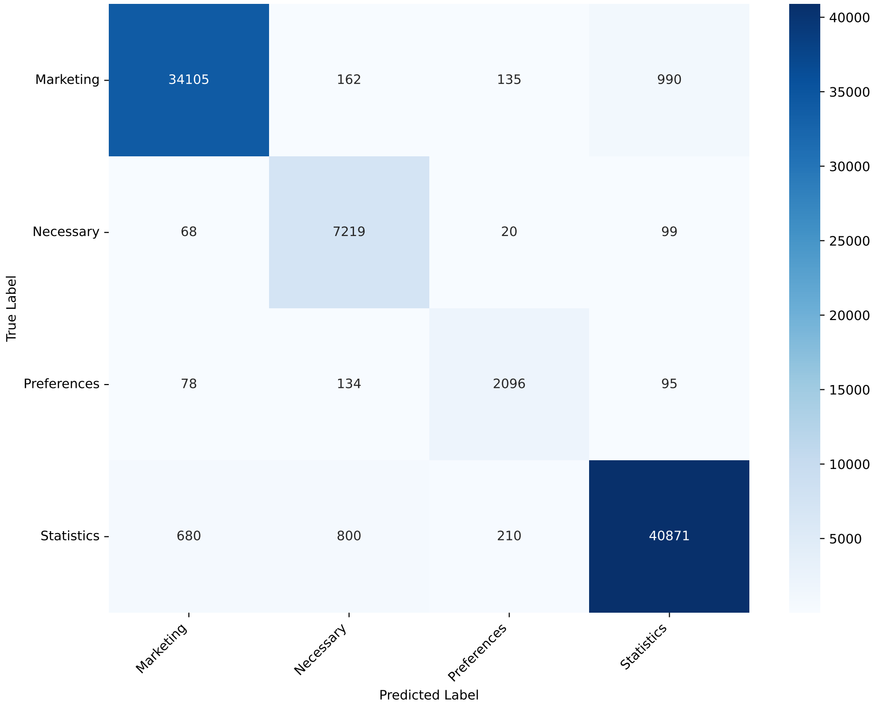
Confusion Matrix - Voting Classifier Test Accuracy: 96.04%
