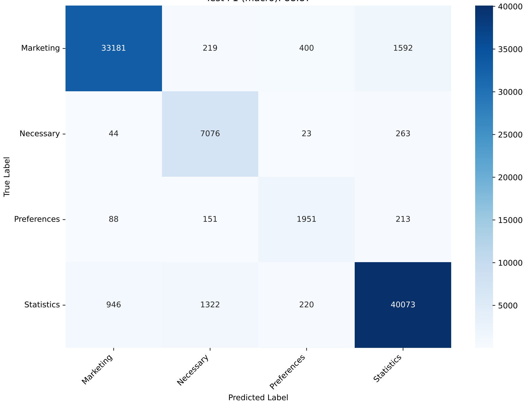
Confusion Matrix - BernoulliNB
