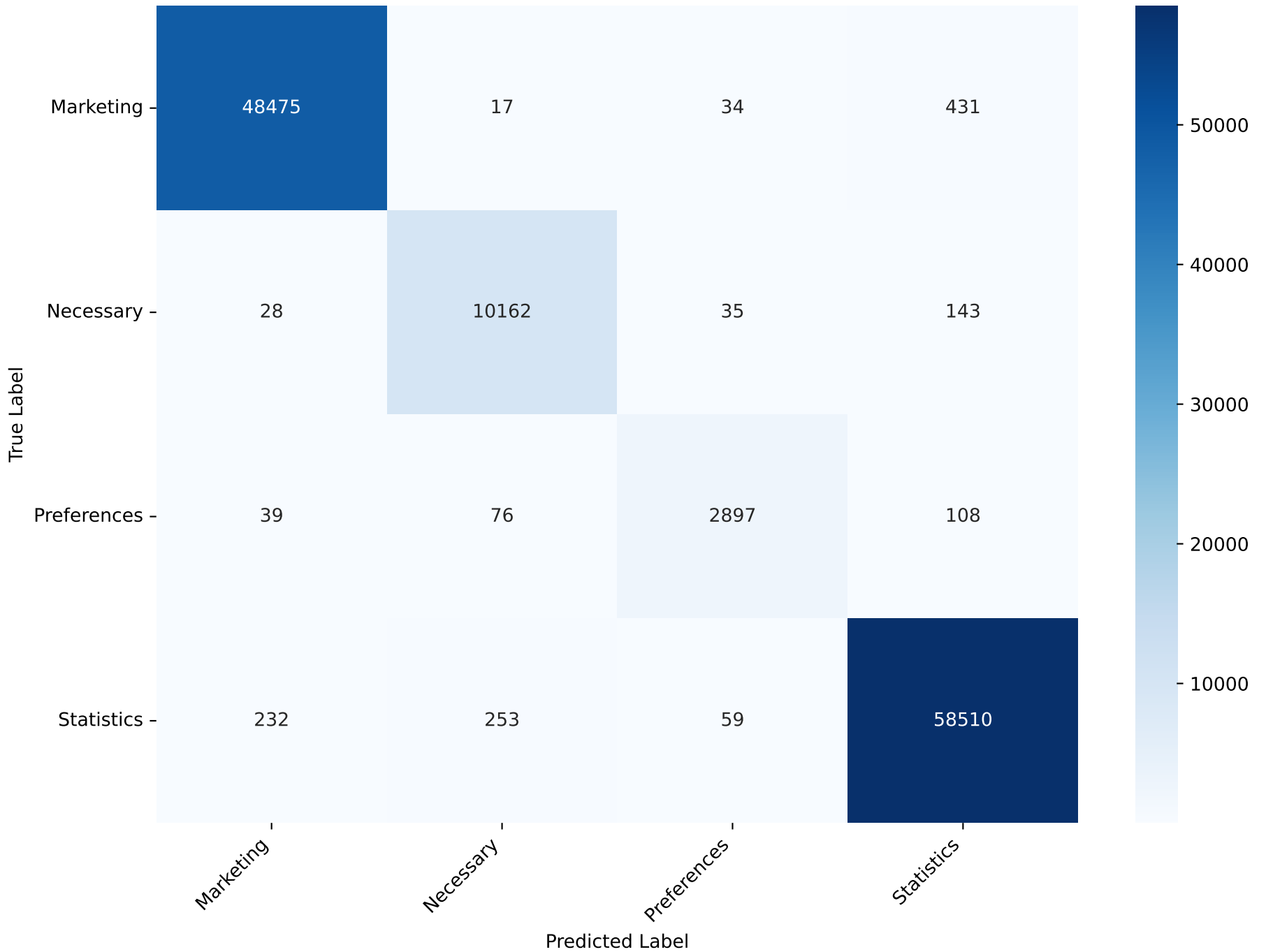
Confusion Matrix - XGBoost Test Accuracy: 98.80% Test F1 (macro): 97.45
