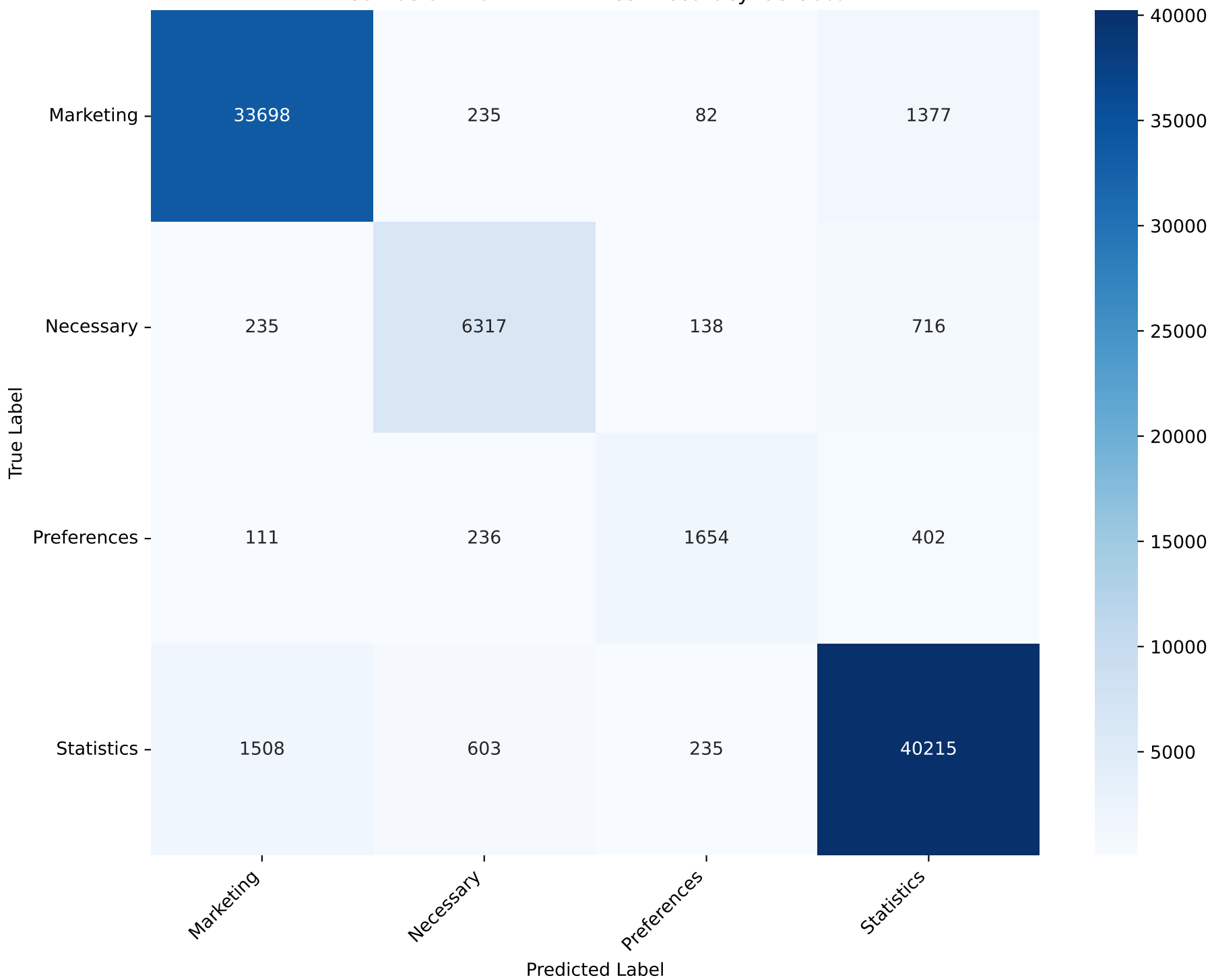
Confusion Matrix - KNN Test Accuracy: 93.30%
