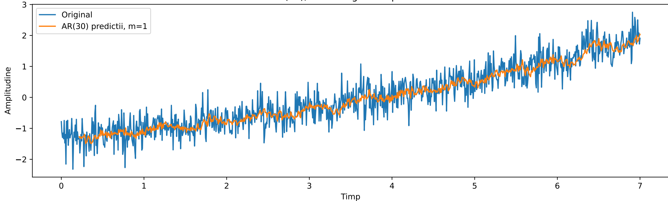
AR(30), m=1: original vs predictii
