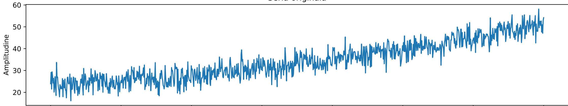
Model MA(q), q = 10
