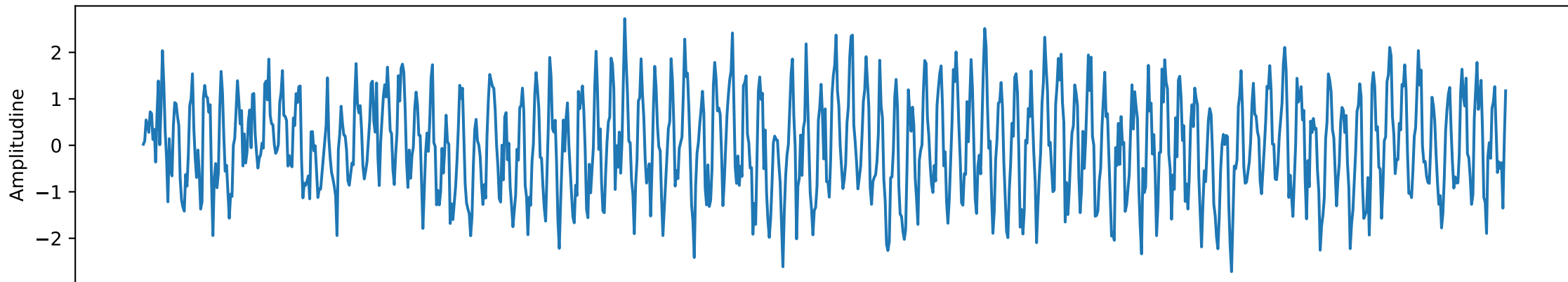
Model ARMA(p, q) cu p = 3 , q = 14
