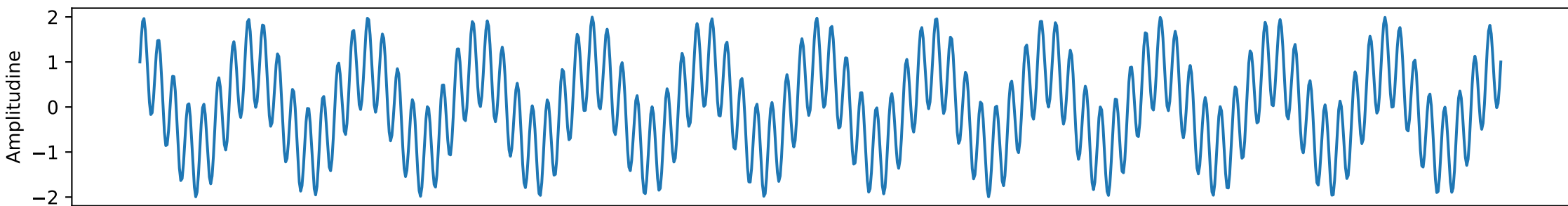
Seasonal
