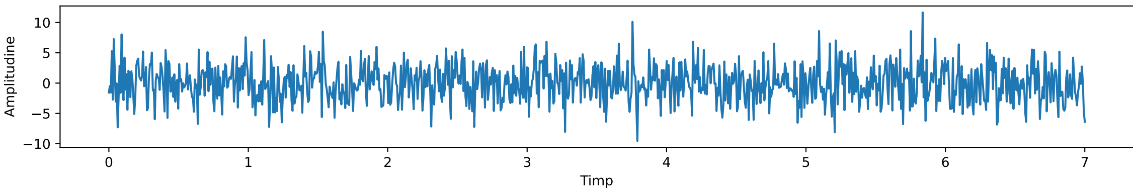
Residuals
