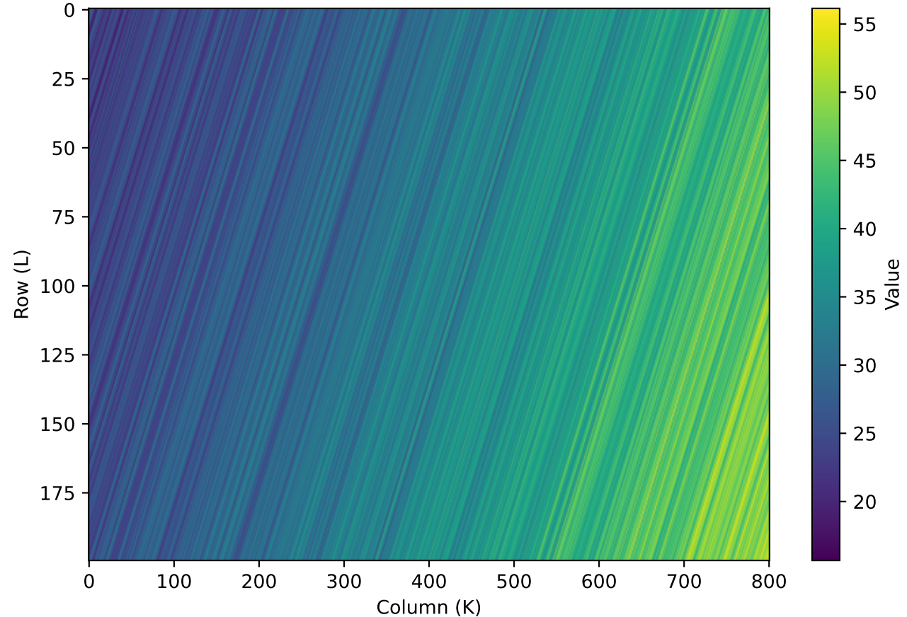
Hankel Matrix
