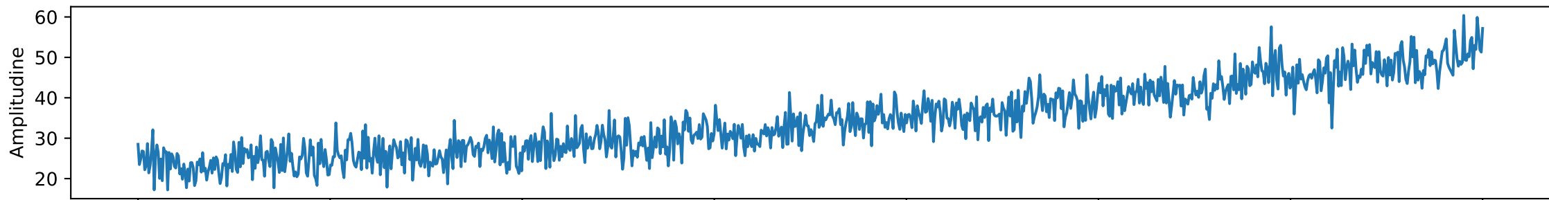
Observed (Trend + Seasonal + Residuals)
