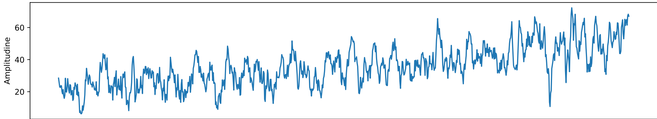
Model MA(q), q = 10
