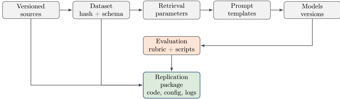
Figure 3: Reproducibility artifact chain. Every experimental result should be traceable to sources, datasets, retrieval settings, prompts, models, parameters, and evaluation procedures.
