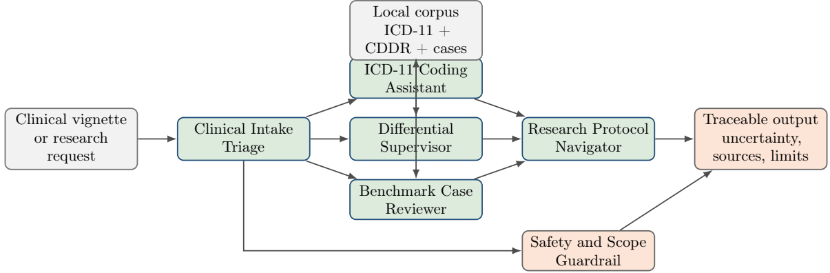
Figure 2: Conceptual multi-agent architecture. Decomposition is not a multiplication of chatbots, but the separation of epistemic responsibilities: case intake, nosological coding, differential diagnosis, benchmark review, protocol navigation, and safety.
