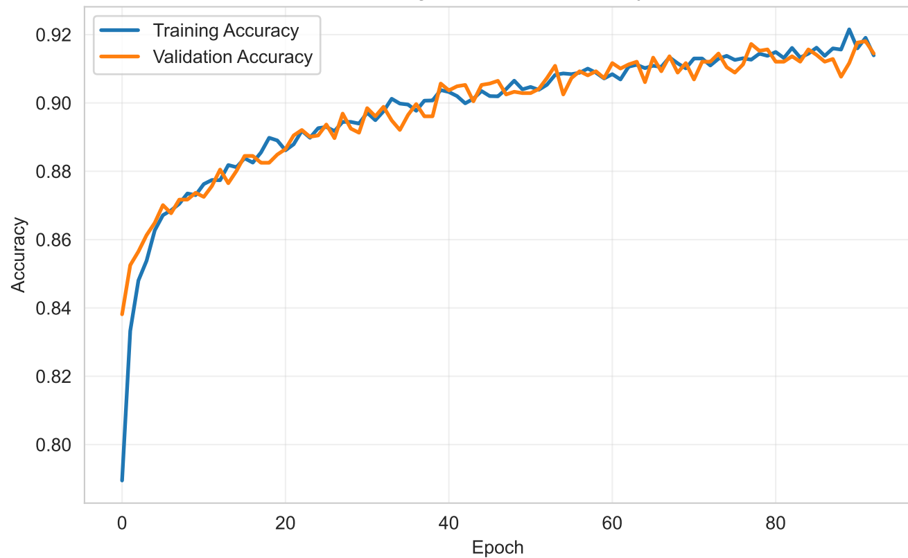
Training & Validation Accuracy
