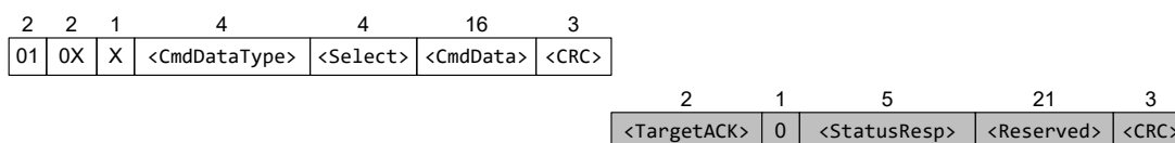
Figure 10. Write Frame Structure
