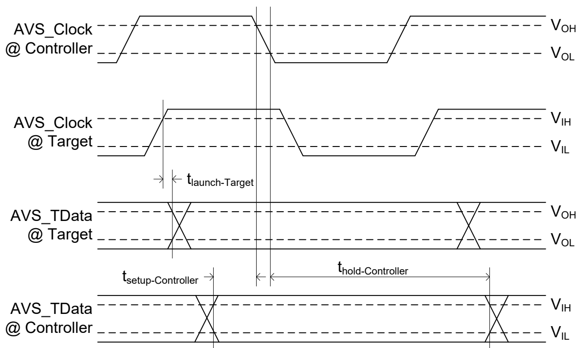
Figure 8. Timing diagram for AVS_TData
