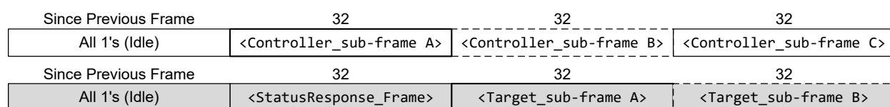
Figure 15. First Frame In A Sequence
