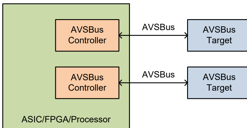
Figure 3. Example AVSBus Topology With Multiple Links
