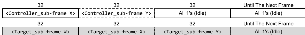
Figure 13. Last Frame In A Sequence.
