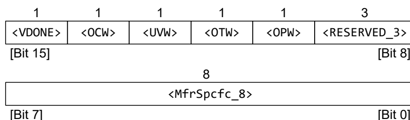
Figure 16. AVSBus_Status_Bits
