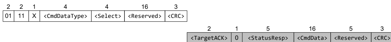
Figure 11. Read Frame Structure
