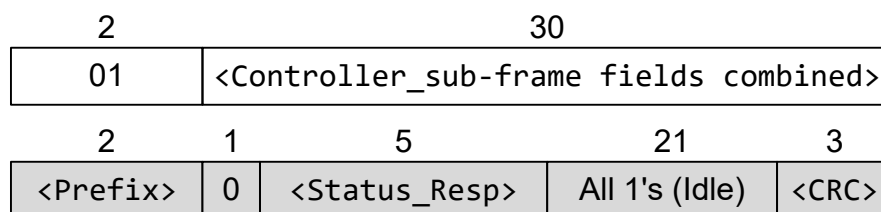
Figure 14. Status Response Frame
