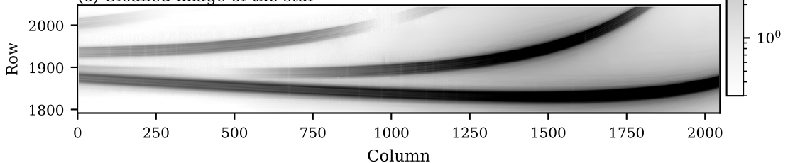
(c) Cleaned image of the star
