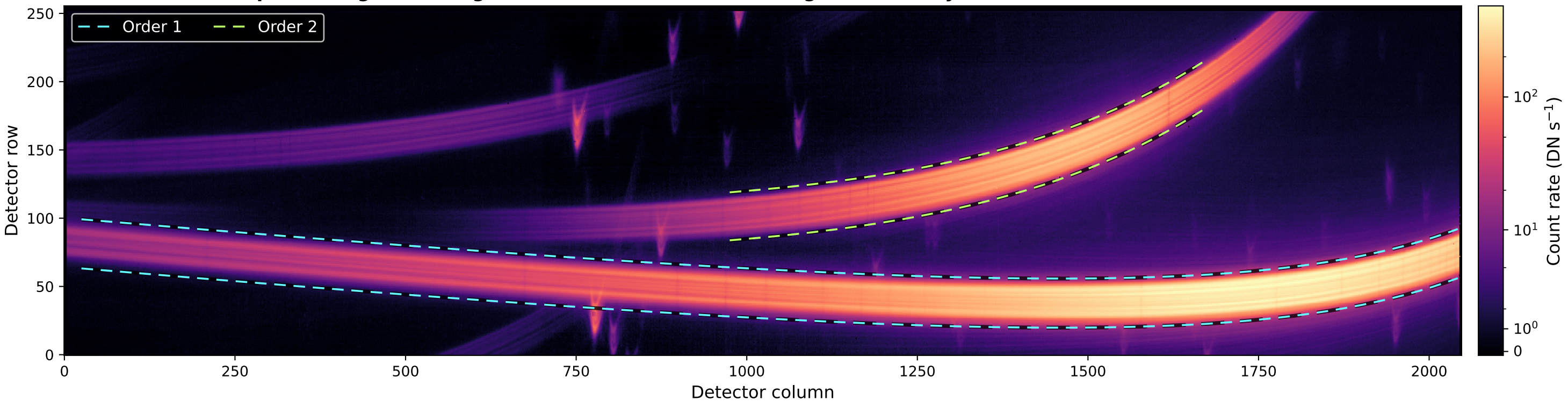
(b) After detector processing and background subtraction, with the regions fitted by NOVA
