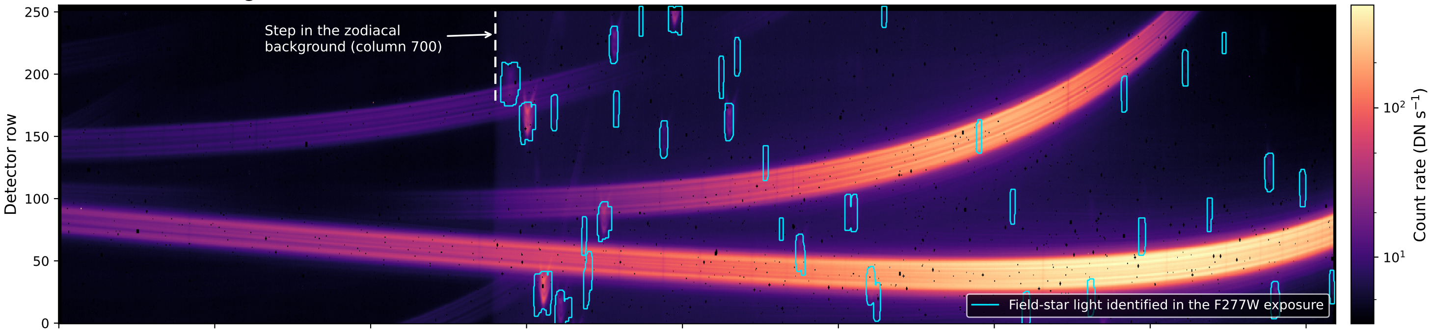
(b) After detector processing and background subtraction, with the regions fitted by NOVA
