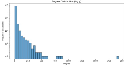
(a) Degree distribution, network reale
