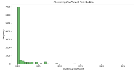
(k) Clustering coefficient locale, Barabasi-Albert
