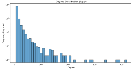
(b) Degree distribution, Barabasi-Albert
