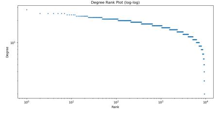
(f) Degree-Rank plot, Erdos-Renyi
