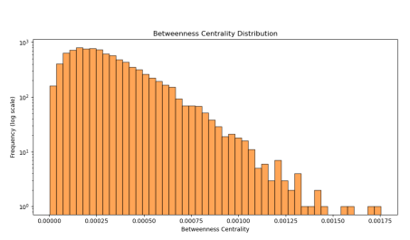
(i) Betweenness centrality, Erdos-Renyi
