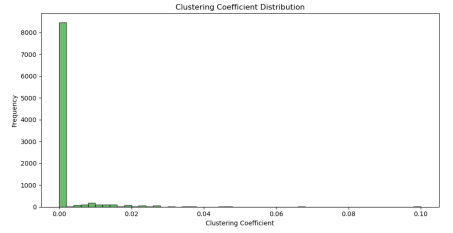
(l) Clustering coefficient locale, Erdos-Renyi
