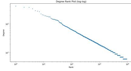
(e) Degree-Rank plot Barabasi-Albert
