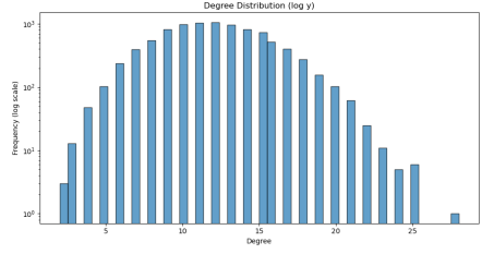
(c) Degree distribution, Erdos-Renyi
