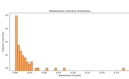
(g) Betweenness centrality, network reale
