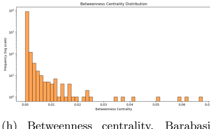
(h) Betweenness centrality, Barabasi-Albert
