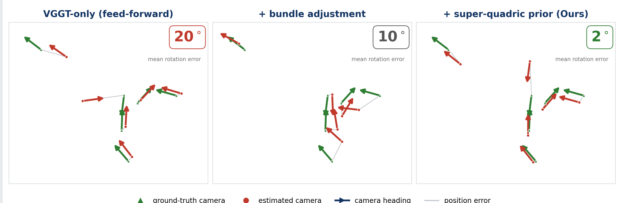
Figure 2: one scene (scene 6, 6 views), cameras Sim(3)-aligned to ground truth for display. Estimated headings (red) move toward ground truth (green) as bundle adjustment, then the prior, are added. Mean rotation error 20^\circ \rightarrow 10^\circ \rightarrow 2^\circ (pose AUC@5 29 \rightarrow 48 \rightarrow 57).
