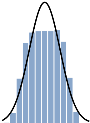
Platykurtic ("thin tails")
