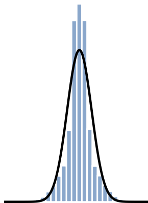
Leptokurtic ("fat tails")
