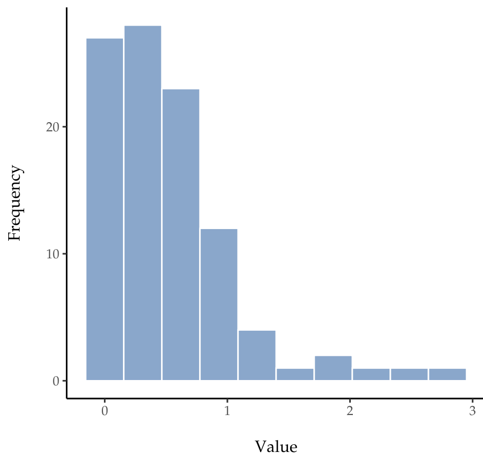
Heavy-Tailed Distributed Data
