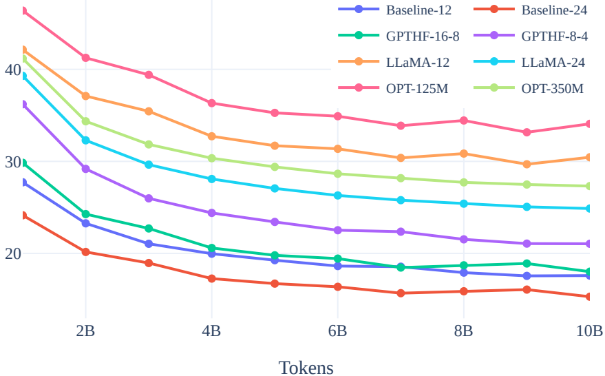
Perplexity
