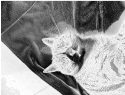
Importance Map
