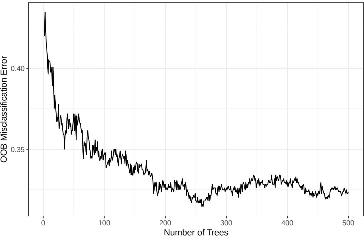
OOB Error vs Number of Trees in Random Forest
