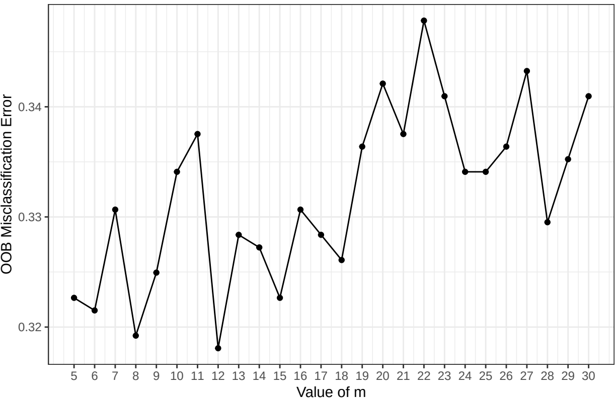
OOB Error vs M tries in Random Forest
