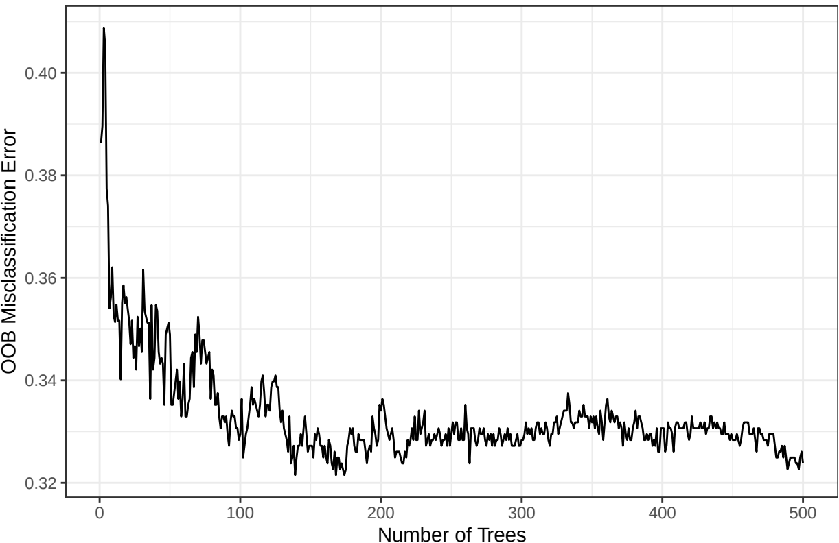
optimal OOB Error vs Number of Trees in Random Forest
