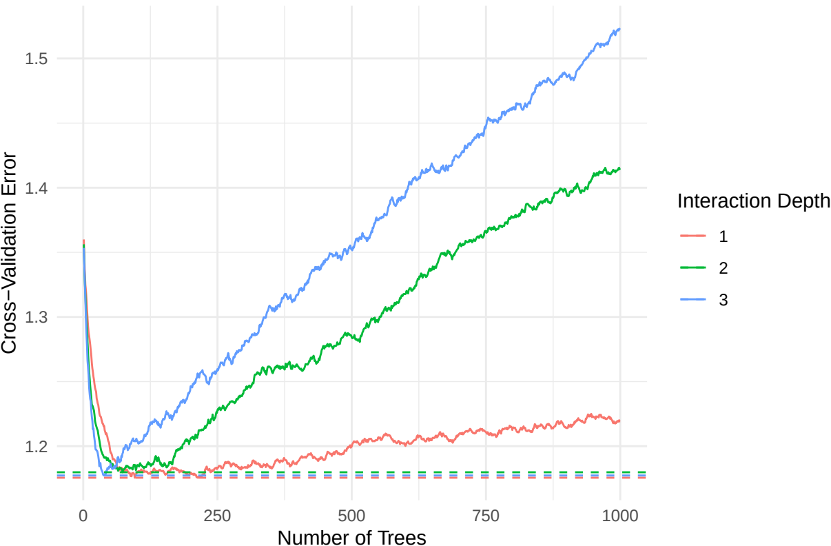
GBM CV Error vs Number of Trees
