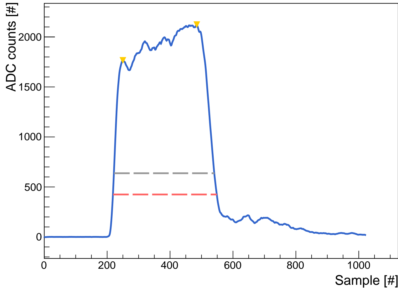
WFtest_run_22100_evt_40_trg_0_ch_4
