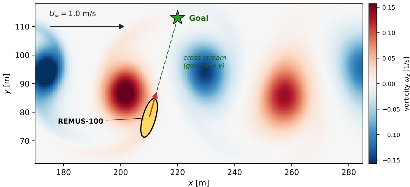
(a) Kármán wake field + REMUS-100 cross-stream task
