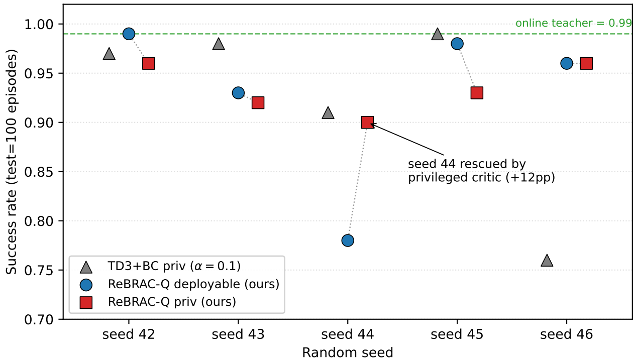
worldcomp-1000: seed-level dispersion across 3 protocols
