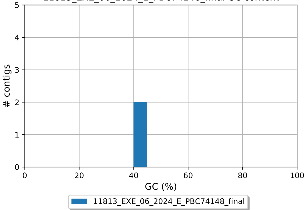
11813_EXE_06_2024_E_PBC74148_final GC content
