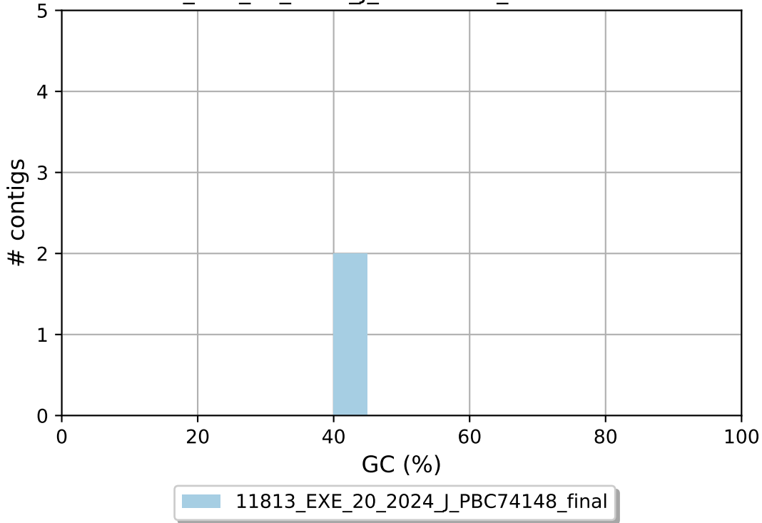
11813_EXE_20_2024_J_PBC74148_final GC content
